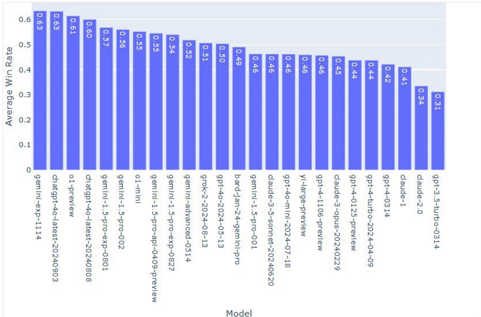
Figure 2: Average Win Rate Against All Other Models (Assuming Uniform Sampling and No Ties)
