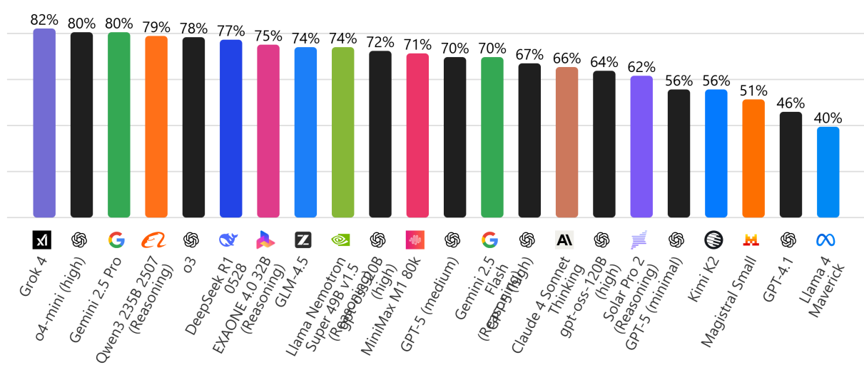
LiveCodeBench (Coding)
