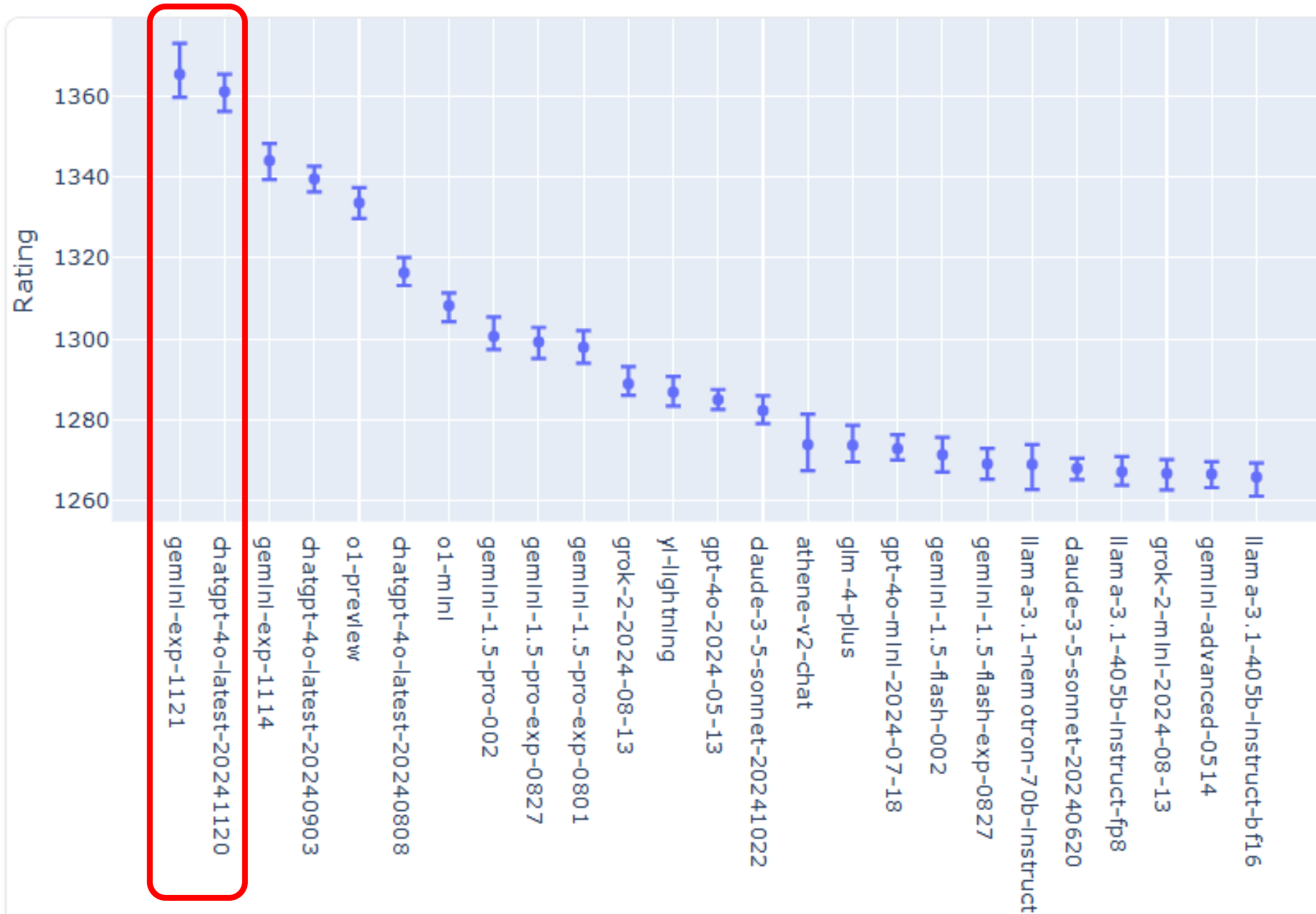
Figure 1: Confidence Intervals on Model Strength (via Bootstrapping)
